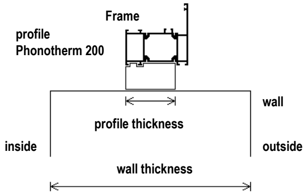
Fig. 1: non-plastered profile
